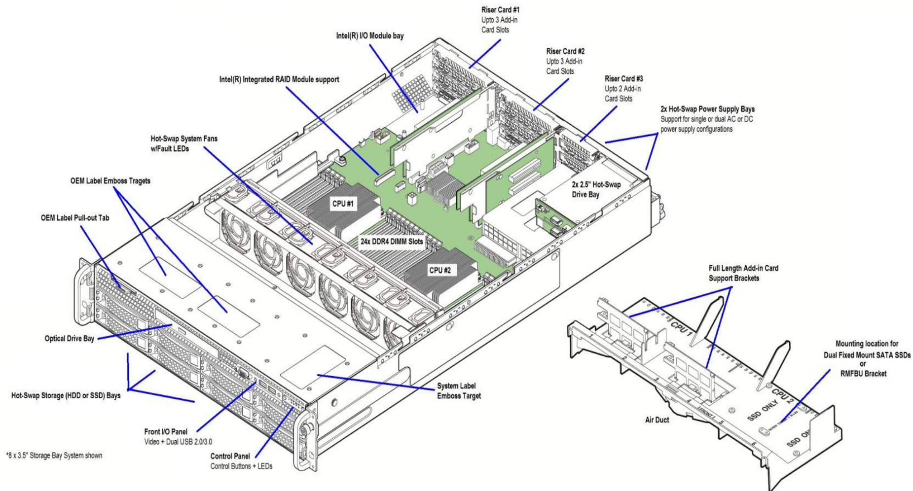
Figure 2. Intel® Server System R2000WT Feature Set Identification
