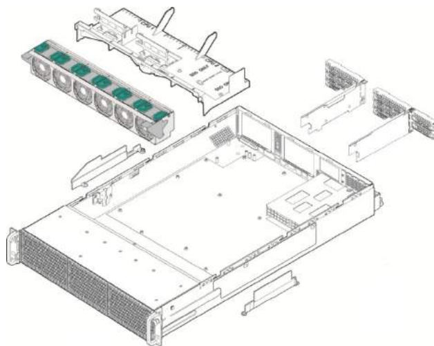
2U – Intel® Server Chassis R2000WT
