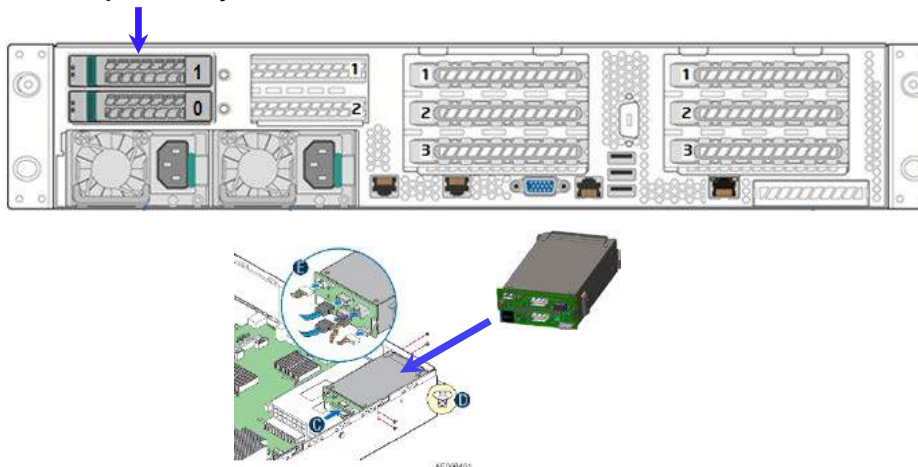
Two 2.5" SATA Hot Swap Drive Bay
